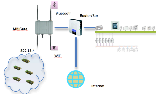
Figure 4. Network architecture of the assisted living environment.
