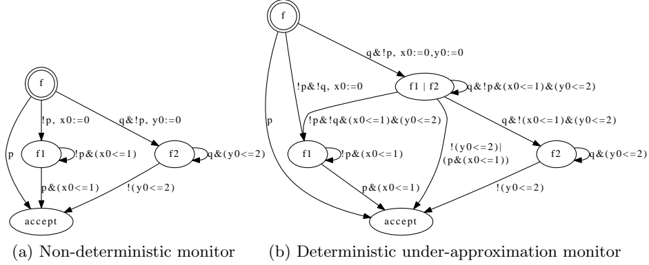
Fig. 2: Monitoring WTA for f \equiv (\diamond_{\leq 1}^x p) \vee (\square_{\leq 2}^y q) , with f1 \equiv (x0 \leq 1) \wedge (true U_{\leq 1-x0}^x p) and f2 \equiv ((c0 \leq 2) \wedge (false R_{\leq 2-y0}^y q)) \vee (y0 > 2) .
