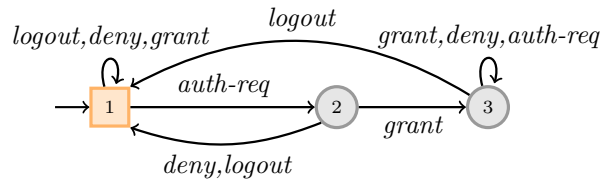
Fig. 7. Some Streett automata for the operating system
