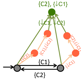
Figure 15: c_1 alternate c_2
