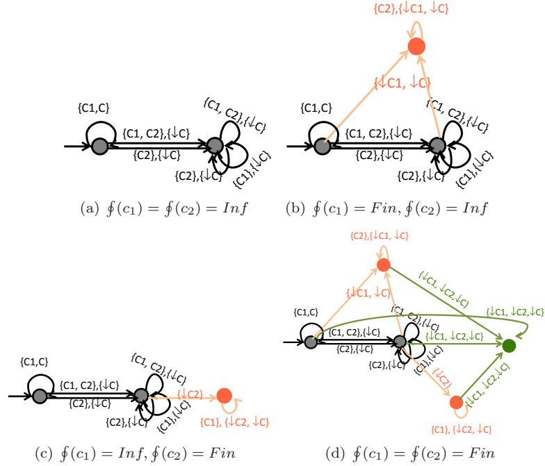
Figure 3: ccAutomata encodings of c = c_1 \text{ upto } c_2
