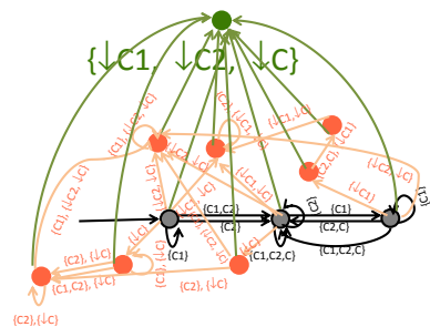
Figure 10: ccAutomata encoding of \text{sampledOn}(\mathcal{J}(c_1) = \mathcal{J}(c_2) = \text{Fin})
