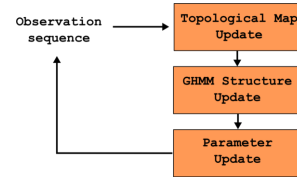
Fig. 2. GHMM learning algorithm overview (adapted from [5])
