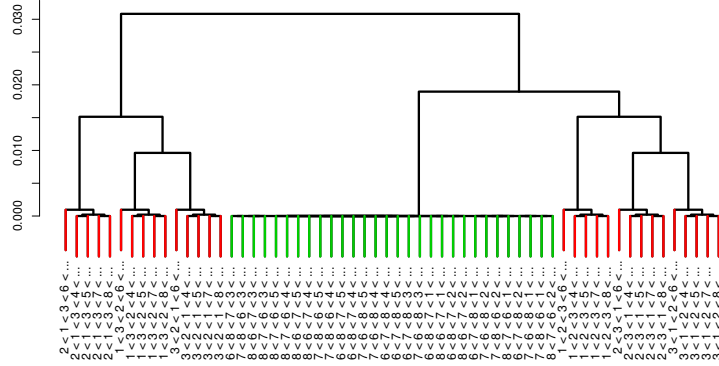
Fig. 4. Dendrogram learned on top- k lists. Red lines (respectively green lines) correspond to examples \mathcal{E}_i = \{\sigma \in \mathfrak{S}_8 : (\sigma_i(i_1), \dots, \sigma_i(i_4)) = (1, \dots, 4)\} with \{i_1, i_2, i_3\} = \{1, 2, 3\} (resp. with \{i_1, i_2, i_3\} = \{6, 7, 8\} ).
