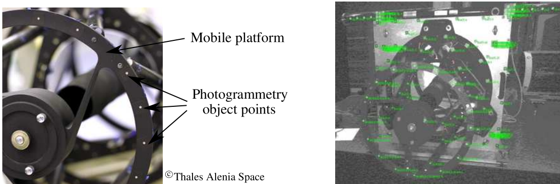
Figure 4: Photo of the telescope mobile platform and photogrammetry data
