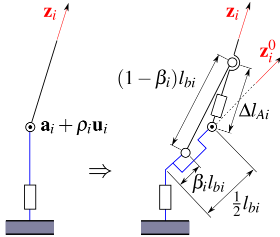
Figure 10: Kinematic model of a flexure joint
