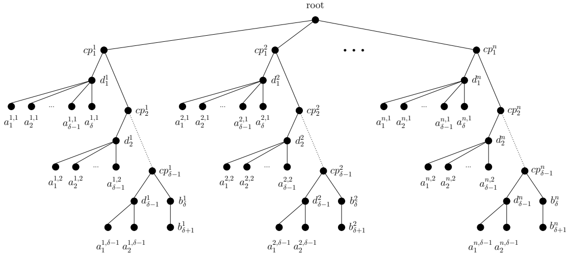
Figure 2: Tree used for establishing Theorem 2.
