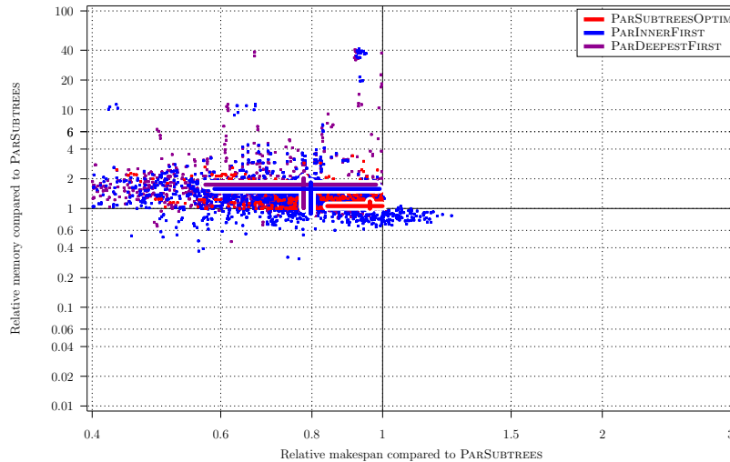
Figure 7: Comparison to PARSUBTREES.
