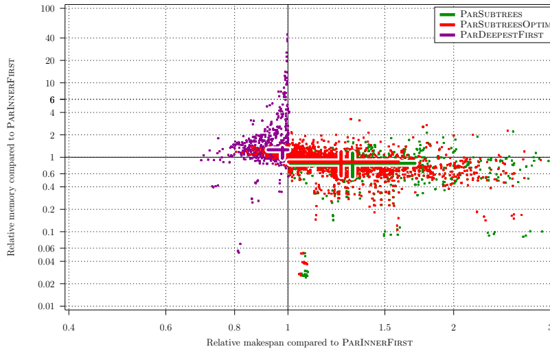
Figure 8: Comparison to PARINNERFIRST.
