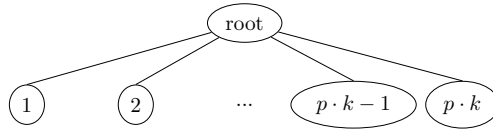
Figure 3: PARSUBTREES is at best a p -approximation for the makespan.
