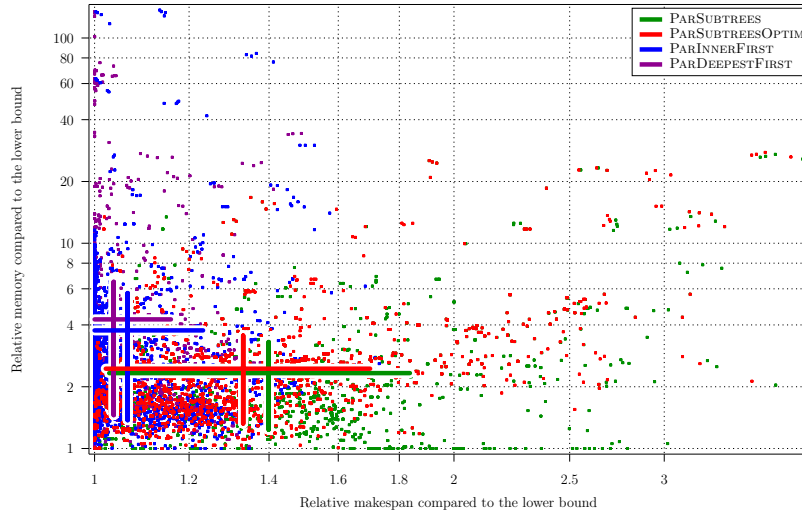
Figure 6: Comparison to lower bounds.
