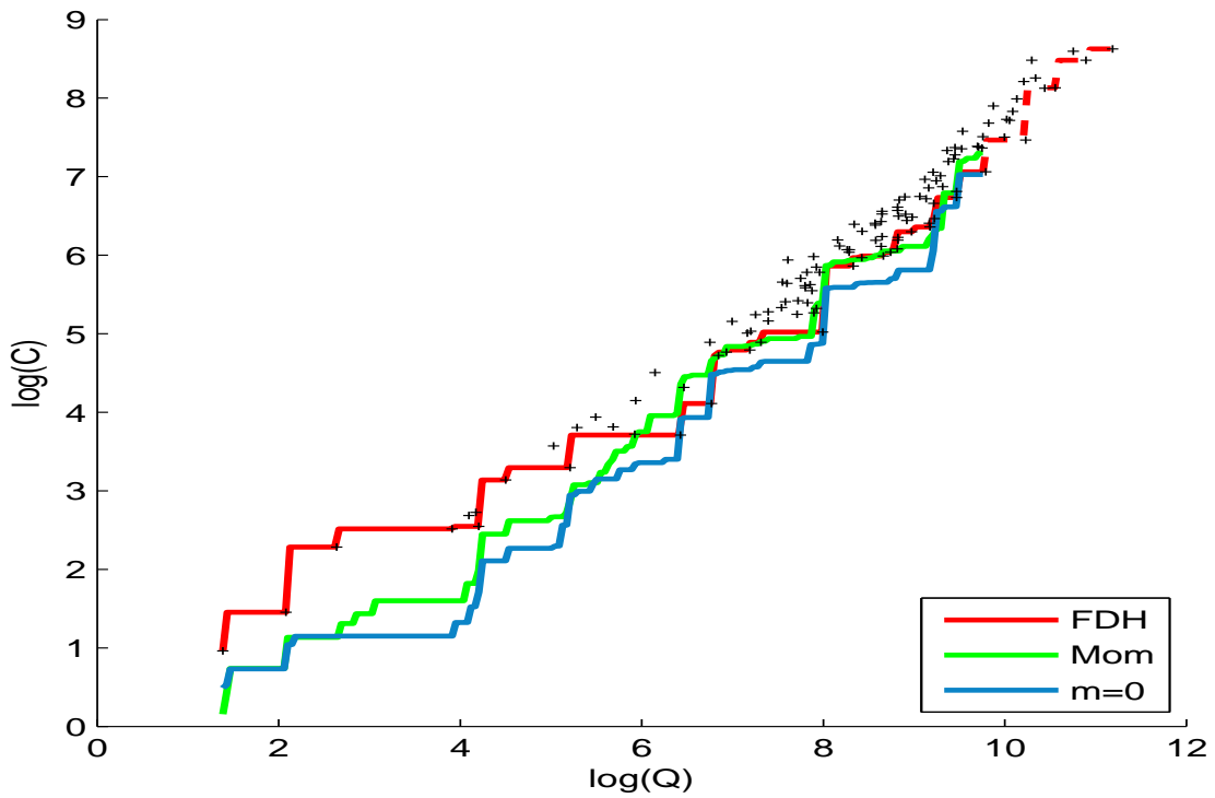
Figure 1: Top — Scatterplot of the 5138 post offices, with the minimum cost function estimators \hat{\varphi}_n (red), \hat{\varphi}_n^\# (green), \tilde{\varphi}_{n,3}^\# (darker blue) and \tilde{\varphi}_{n,6}^\# (lighter blue). Bottom — The 123 electric utility data, with the frontier estimators \hat{\varphi}_n (red), \hat{\varphi}_n^\# (green) and \tilde{\varphi}_{n,0}^\# (blue).
