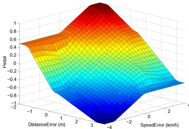
Fig. 8. Control surface for the fuzzy control system.
