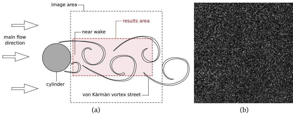
Figure 10: Configuration of the cylinder wake experiment (10a); a 256 \times 256 pixels sub-region (1/16 of the total area) of a sample of PIV image (10b).
