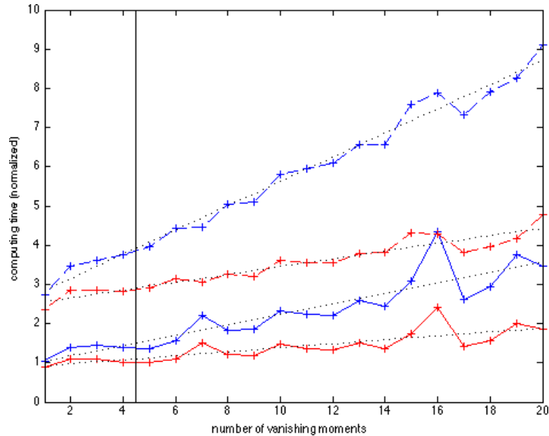
Figure 8: Experiments on the influence of the number of VM on the estimation computing time, using usual filter banks (blue) or “smart” ones (red), for (L, C) = (6, 5) (solid line) and (6, 0) (dashed line). Estimated motions are almost the same, in terms of RMSE, for any number of VM n > 4 , any of the two couples (L, C) and of course any of the filter bank employed – the part of the graph located right of the vertical black line. Computation times are normalized w.r.t. optimum parameters, i.e. (L, C) = (6, 5) , n = 5 and smart filter bank. This reference time corresponds to 9 seconds. Using usual filter banks, the computational burden rapidly increases with the number of VM, especially with low C (dashed blue line). This can be tempered by the use of smart filter banks (dashed red) and/or by choosing a higher value for C (solid lines).
