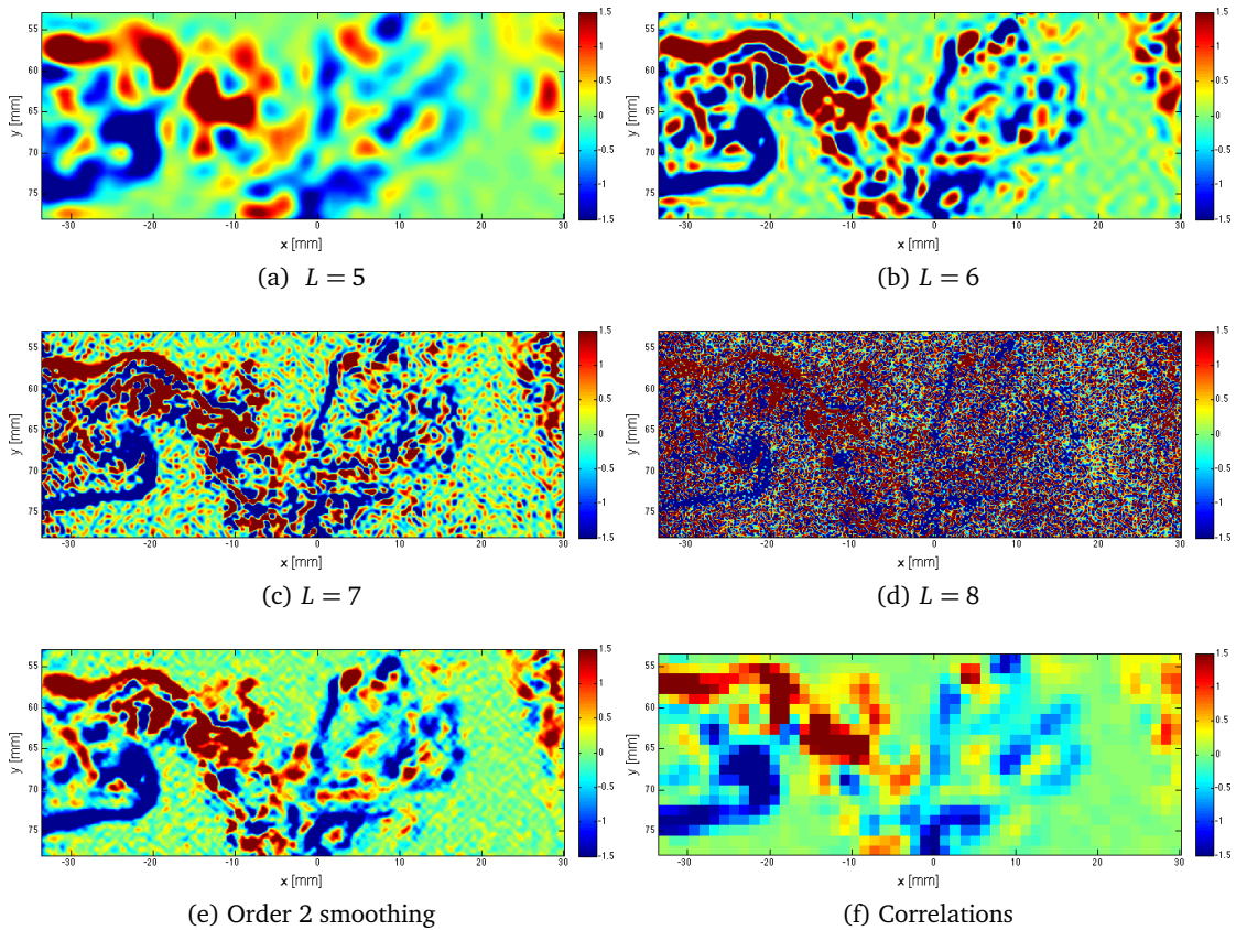
Figure 11: Vorticity comparison. Estimates (11a), (11b), (11c), (11d) are obtained with proposed estimator, varying parameter L . Motion (11e) is obtained with a more evolved estimator featuring explicit smoothing terms [10]. Last estimate (11f) is a reference given by the correlation-based method.
