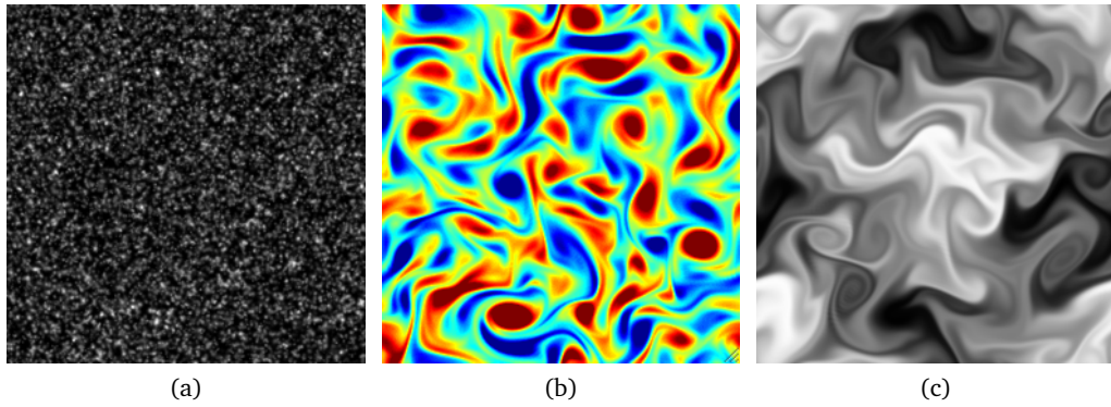
Figure 3: The first frame of the synthetic PIV image sequence (3a) with the vorticity of the underlying reference velocity field \mathbf{v}_{\text{ref}} (3b). A sample frame from the synthetic passive scalar advection-diffusion sequence (3c).
