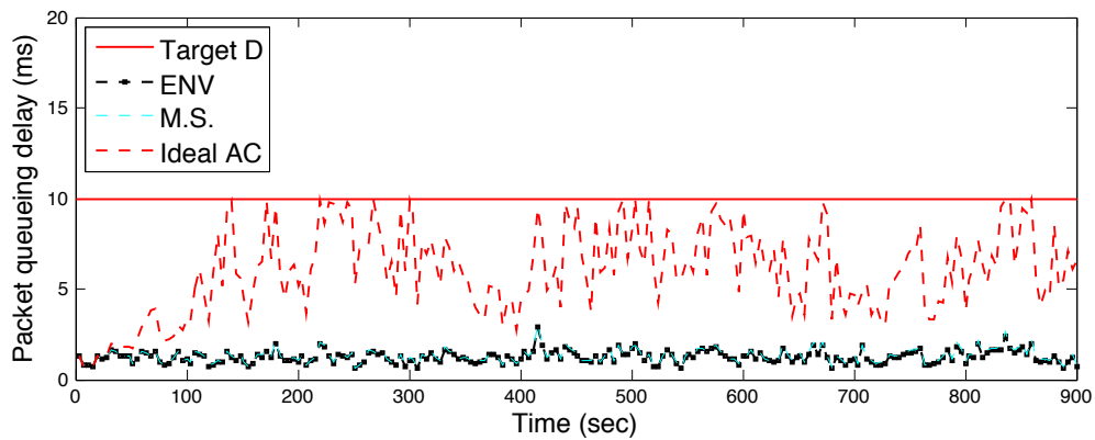
Figure 5: Real traffic trace for the initial background traffic
