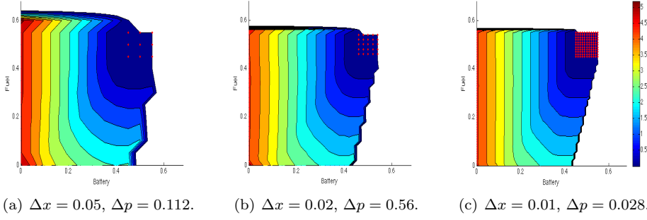
FIGURE 4.1. Test 1. Contour plots of the minimum time function: Three discretization steps in \Delta x and \Delta p .
