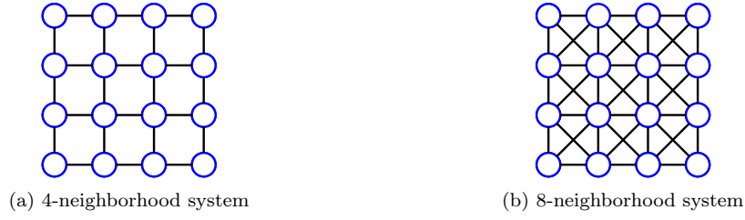
Figure 3: Examples of MRFs with Grid-like Structures
