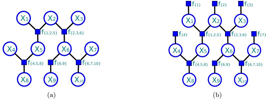
Figure 2: Examples of Factor Graphs. Note that both of the Bayesian Network in Fig. 1(a) and the Markov Random Filed in Fig. 1(b) can be represented by the two factor graphs above. Nevertheless, the factor graph in (b) contains factors corresponding to non-maximal cliques.
