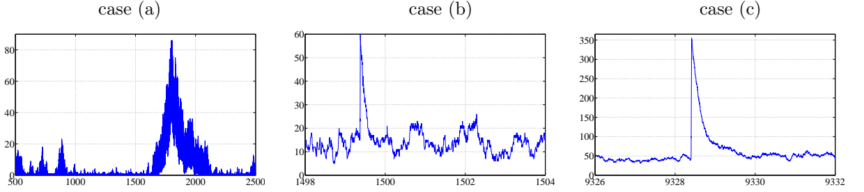
FIGURE 4 – Illustration of our model ability at generating different dynamics of workload I(t) . See Table 1 for the parameter values corresponding to each of these three cases. The X -axis corresponds to time (in hours unit) while the Y -axis indicates the number of active viewers.
