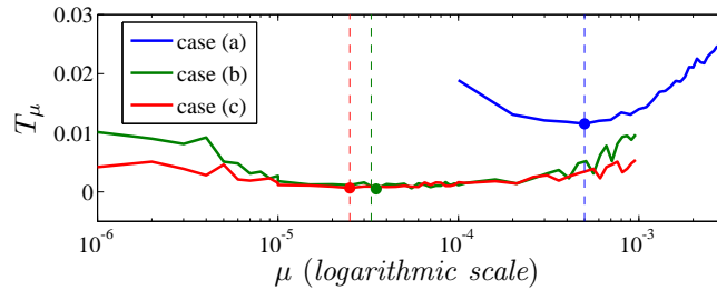
FIGURE 5 – Evolution of the exponential test statistics (10) applied to the traces of Figure 4. Dotted vertical lines locate the actual value of \mu for each case ; dot markers on each curve indicate the estimated value \hat{\mu} corresponding to the minimum point of the statistical test T_\mu .
