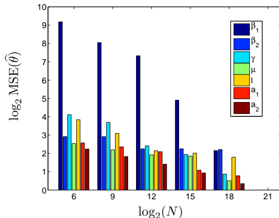
FIGURE 9 – Evolution of the Mean Square Error versus the data length N in a log-log plot. For the sake of conciseness, we only show here the results corresponding to the case (b) of Table 1.
