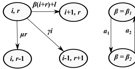
FIGURE 3 – Markov chain diagram representing the evolution of the Current viewers ( i ) and Past Viewers ( r ) populations with a Hidden Markov Model.
