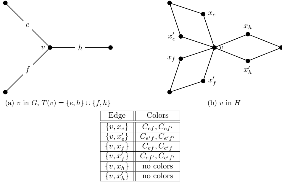
Figure 6: Color assignment for vertices with degree 3.
