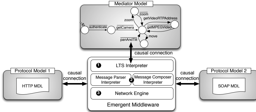
Fig. 7 Runtime models building an emergent middleware
