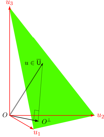
Figure 2: Construction of orthogonal vectors in MGDA-II
