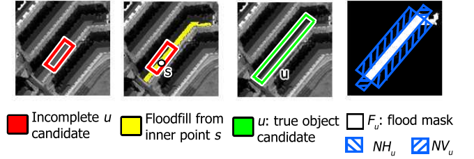
Fig. 12. Floodfill based feature for roof completeness
