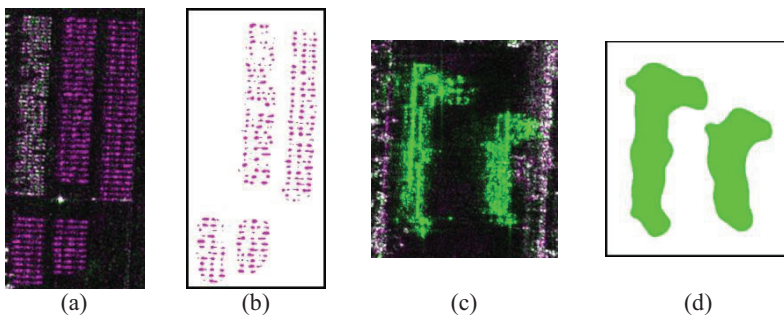
Fig. 4 RGB multitemporal composition (R:04/24/2010, G:04/23/2010, B:04/24/2010) and CD map of two full-scene sub-sets (COSMO-SkyMed Product – ©ASI – Agenzia Spaziale Italiana –2010) showing (a-b) cargo terminal where new cars were stocked and (c-d) a wet dock zone where two cargo ships were anchored.
