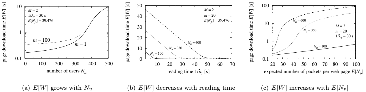
(a) E[W] grows with N_u
