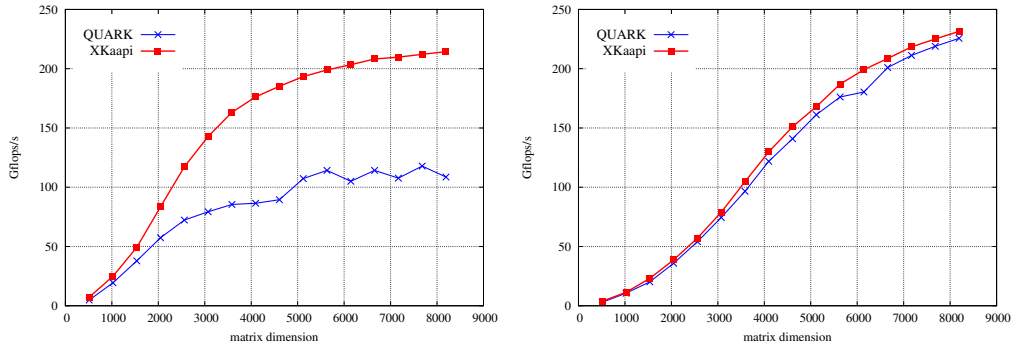
Figure 2: Gflops on Cholesky algorithm with QUARK and X-KAAPI. Tile size of NB = 128 (left) or NB = 256 (right).
