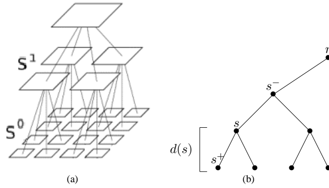
Fig. 1. (a) Hierarchical model structure: quad-tree; (b) Quad-tree notations.
