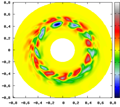
Figure 21: Poloidal cut of electric potential at different time steps ( t = 1600 left, t = 4800 right), \varphi = 0 , BSL scheme
