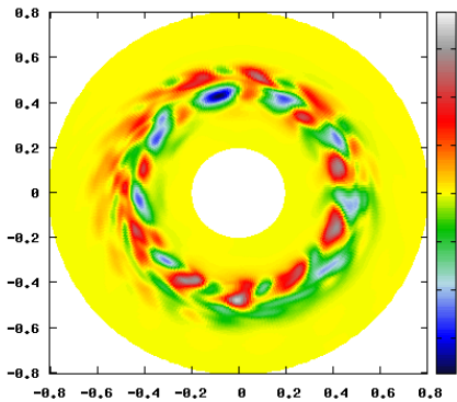
Figure 22: Poloidal cut of electric potential at different time steps ( t = 1600 left, t = 4800 right), \varphi = 0 , FSL scheme
