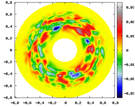
Figure 21: Poloidal cut of electric potential at different time steps ( t = 1600 left, t = 4800 right), \varphi = 0 , BSL scheme
