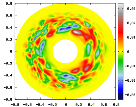
Figure 22: Poloidal cut of electric potential at different time steps ( t = 1600 left, t = 4800 right), \varphi = 0 , FSL scheme
