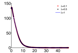
Fig. 8. Behavior of the kinetic energy density for different values of \lambda ( x axis in second).
