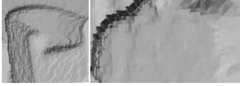
(a) Dense surface reconstruction using the disparity map D_p corresponding to a 2D triangulation of the ToF data points. Zoomed sofa chair (left) and zoomed T-shirt (right) from SET-2 in fig. 5.7(b).
