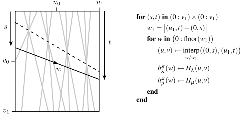
Fig. 3.4 A line h_k^{st}(w) , with end-points (0,s) and (u_1,t) , is swept through each Hough transform H_k . A total of v_1 \times v_1 1-D histograms h_k^{st}(w) are computed in this way. See section 3.3.6 for details.
