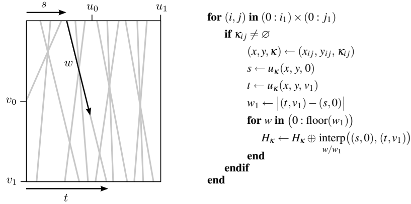
Fig. 3.3 Hough transform. Each gradient pixel (x, y) labelled \kappa \in \{\lambda, \mu\} maps to a line u_\kappa(x, y, v) in transform H_\kappa . The operators H \oplus p and \text{interp}_\alpha(p, q) perform accumulation and linear interpolation, respectively. See section 3.3.5 for details.
