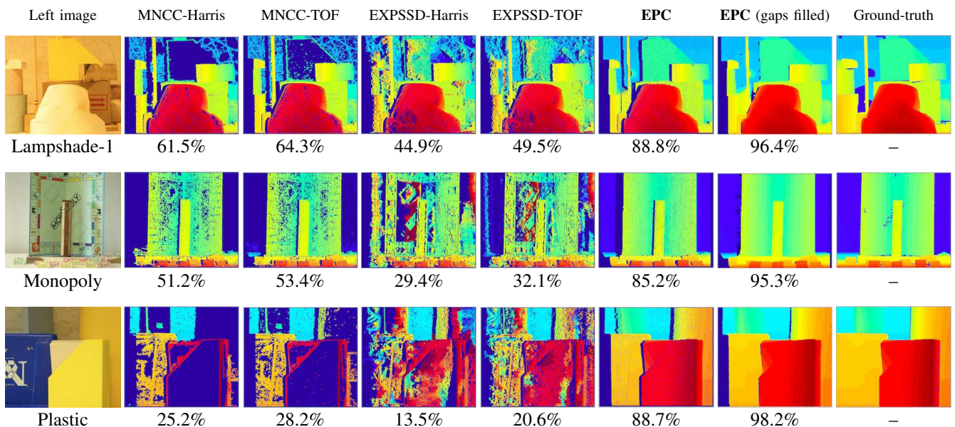
Fig. 9. Middlebury dataset. We show left images, results of the same algorithms as in Fig. 6 and 7, and the ground-truth disparity maps. There are error statistics (percentage of correctly matched pixels) below the disparity maps. Observations from the real-world cases are confirmed quantitatively. The algorithm using the full model (EPC) gives clearly the best results.
