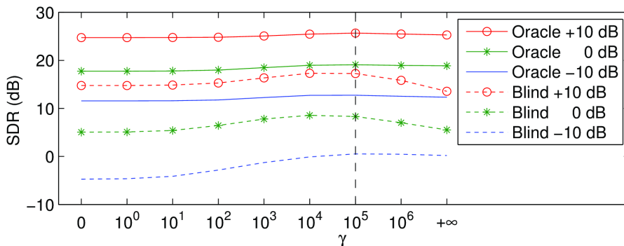
Figure 2: Output SDR of the classical Wiener filter ( \gamma = 0 ) and the proposed constraint-based ( \gamma = +\infty ) and penalty-based algorithms in oracle and blind conditions, averaged over all mixtures for each input SNR.
