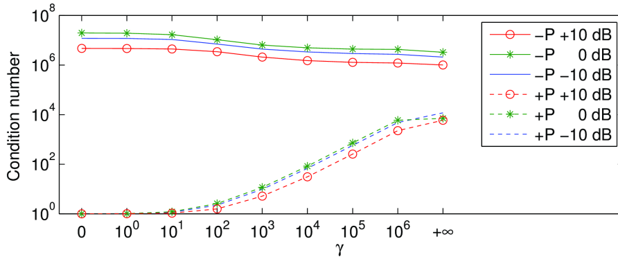
Figure 1: Condition numbers of the linear systems (11) and (15) in oracle conditions with (+P) and without (-P) preconditioning, for the classical Wiener filter ( \gamma = 0 ) and for the proposed constraint-based ( \gamma = +\infty ) and penalty-based algorithms, averaged over all mixtures for each input SNR.
