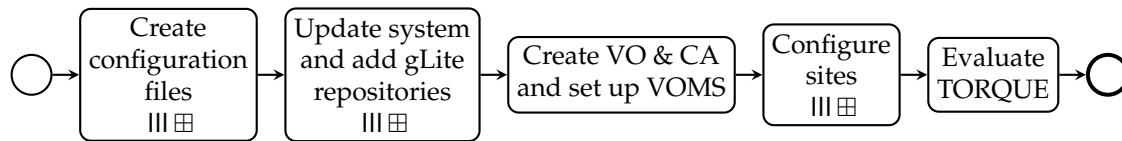
Figure 2: A workflow representation of gLite experiment. The nodes marked with III symbol represent subprocesses executed in parallel (☐ symbol depicts a collapsed subprocess). The workflow features the deployment of the experiment as it is the most complex part. The abbreviations (VO, CA, VOMS) are names of gLite services. TORQUE is the evaluated batch scheduler.
