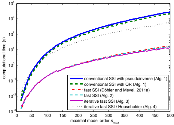
(a) r = 251, r_0 = 5, c \approx 50
