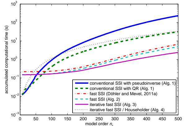
(b) r = r_0 = 5, c \approx 1
