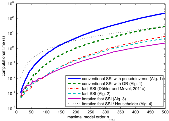
(b) r = r_0 = 5, c \approx 1
