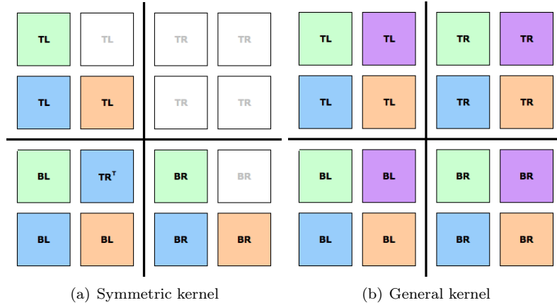
Figure 2: SRBT core kernel ( B_i^T A_{ij} B_j ), data dependencies among tiles of A_{ij} , given by matching colors.
