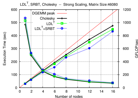
Figure 11: Strong Scaling using a 46080x46080 matrix
