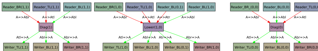
Figure 6: SRBT DAG for 4x4 tile matrix
