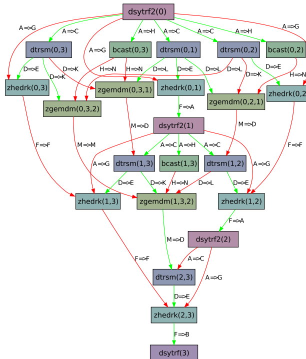
Figure 8: LDL^T DAG for 4x4 tile matrix
