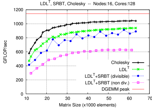
Figure 10: Problem Scaling (Flops) on a 16 \times 8 = 128 core cluster
