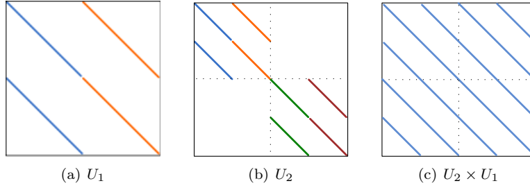
Figure 1: Sparsity pattern of matrix U .
