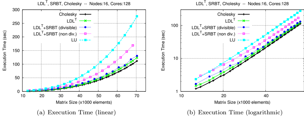
Figure 9: Problem Scaling comparison of \text{LDL}^T + \text{SRBT} against Cholesky on a 16 \times 8 = 128 core cluster
