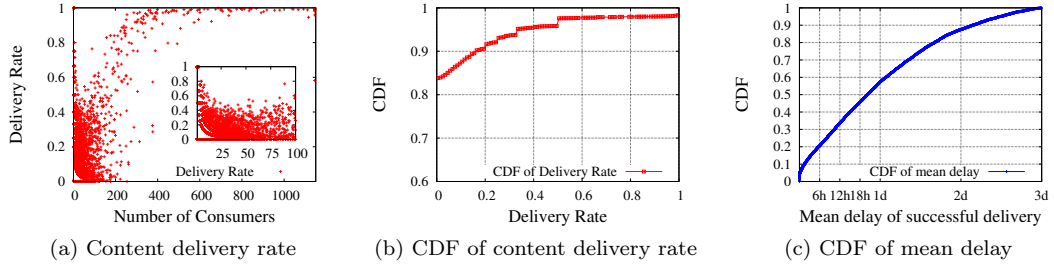
Figure 2: Effectiveness of opportunistic communication in content dissemination in mobile social networks
