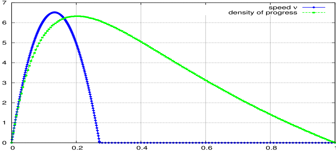
Fig. 2. Comparison of mean speed in the NN model and density of progress
