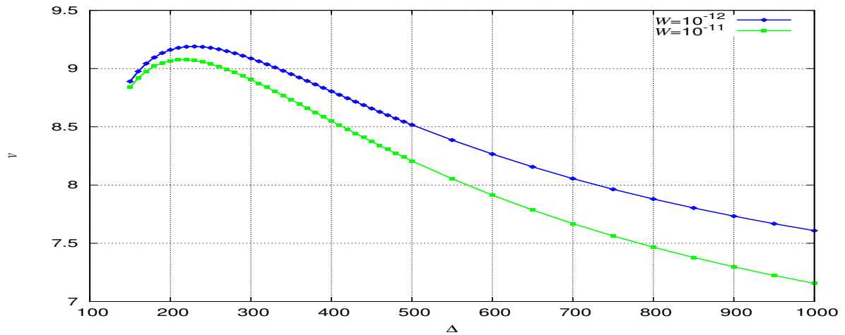
Fig. 9. Mean long-distance speed with respect to \Delta for W = 10^{-11} and W = 10^{-12} .
