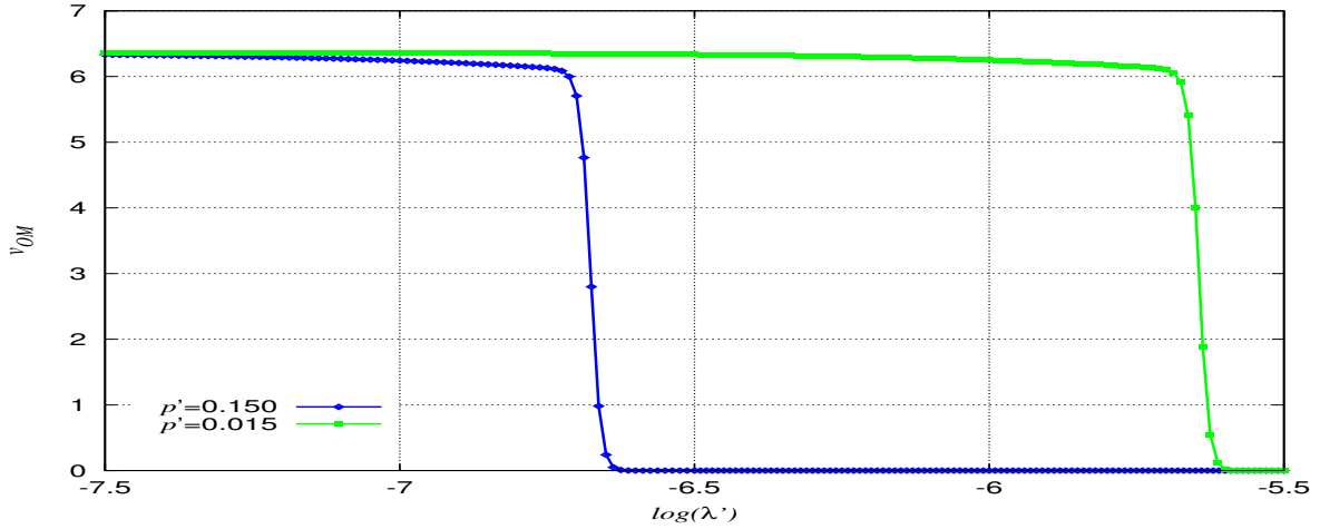
Fig. 7. Mean short-distance speed with respect to the spatial intensity of the field of interferers \lambda' , M = 10000
