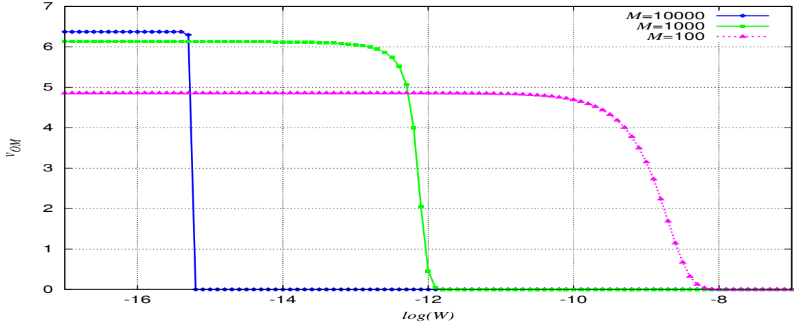
Fig. 6. Mean short-distance speed with respect to noise W in the NN model.
