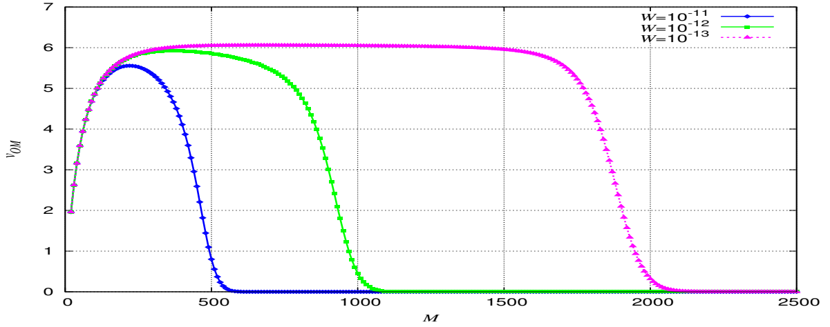
Fig. 5. Mean short-distance speed with respect to the distance M in the NN model, W = 10^{-11}, 10^{-12}, 10^{-13} .
