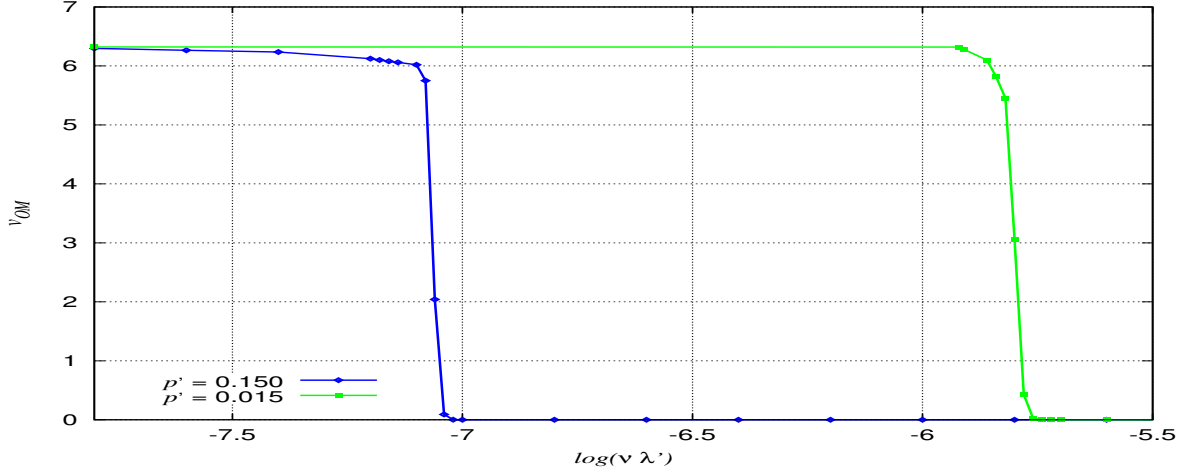
Fig. 8. Mean short-distance speed with respect to the spatial intensity \nu\lambda' of Poisson-line process, M = 10000
