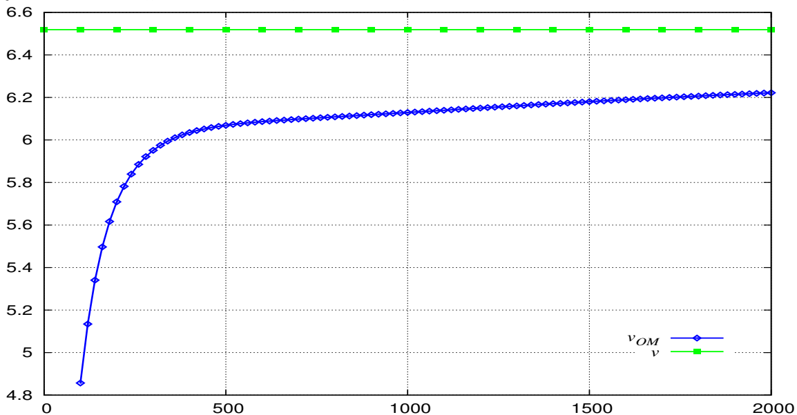
Fig. 4. Mean short-distance speed v_{OM} with respect to M in the NN model and long-distance speed v .
