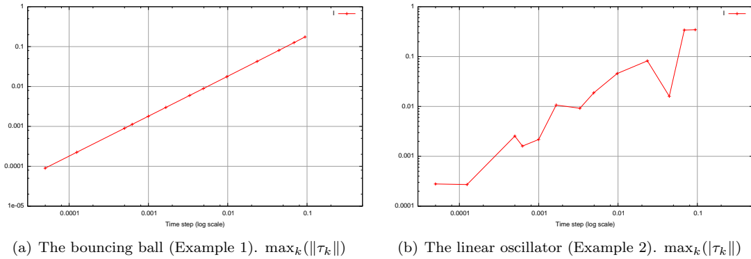
Figure 3: I) Magnitude of the multiplier \tau_{k+1} with respect to the time step size for the direct projected scheme (28).
