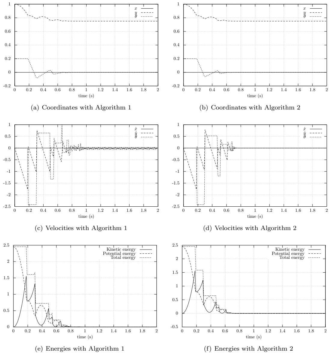
Figure 9: The Rocking Block (Example 3). Comparison of the direct projection scheme (Algorithm 1) and the combined activation/projection approach (Algorithm 2).
