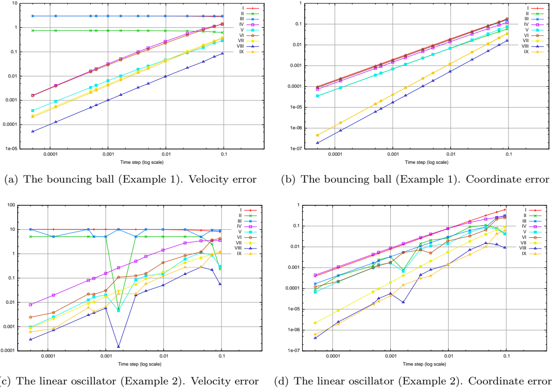
Figure 2: Empirical order of convergence of time-stepping schemes. Paoli–Schatzman scheme: I) uniform norm, IV) l_1 norm, VII) l_2 norm. Moreau–Jean’s scheme: II) uniform norm, V) l_1 norm, VIII) l_2 norm. Direct projected scheme (28). III) uniform norm, VII) l_1 norm, IX) l_2 norm.
