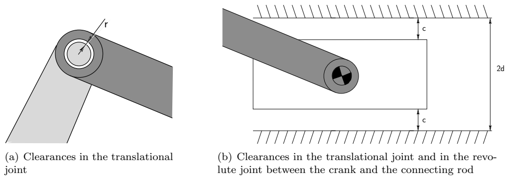
Figure 22: Details of the clearance modeling
