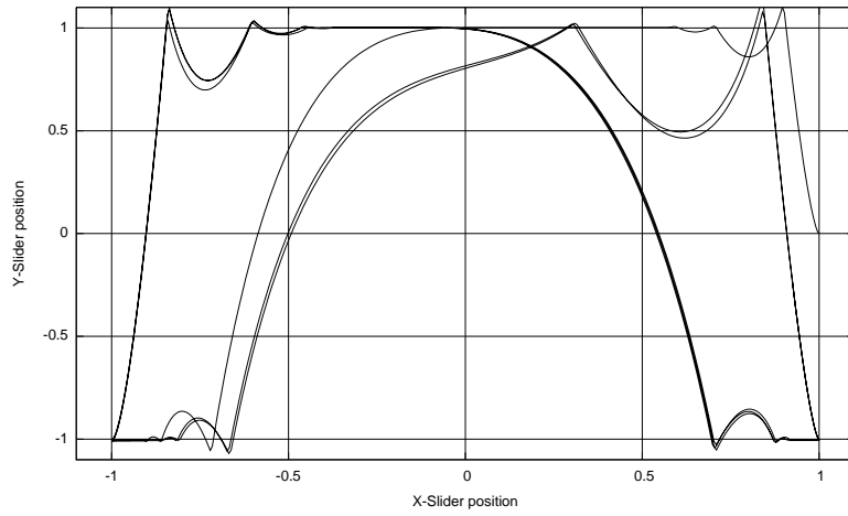
(a) slider portrait with Moreau–Jean’s scheme (18d)
