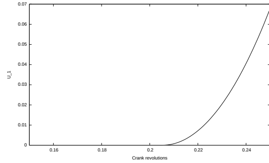
(b) Moreau-Jean's scheme (18d) on [0.15, 0.25] .
