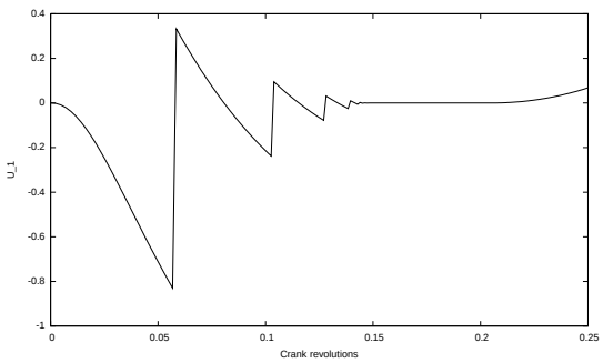
(e) Combined scheme (Algorithm 2) on [0, 0.25] .
