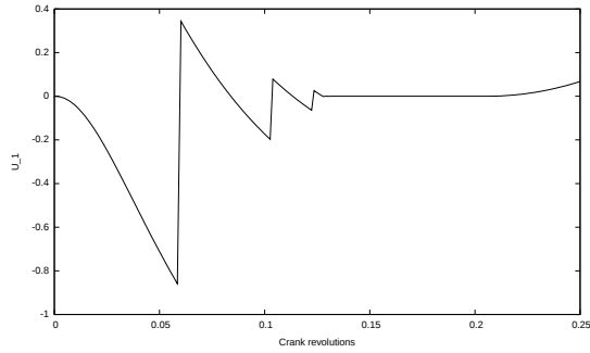
(a) Moreau-Jean's scheme (18d) on [0, 0.25] .
