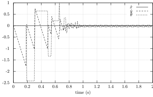
(c) Velocities with Algorithm 1
