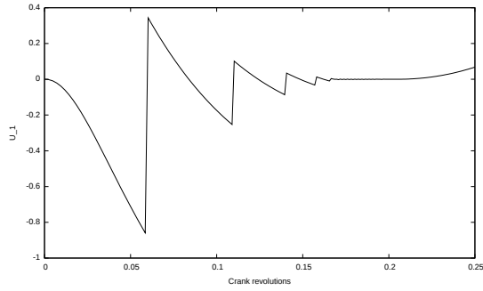
(c) Direct projected scheme (Algorithm 1) on [0, 0.25] .
