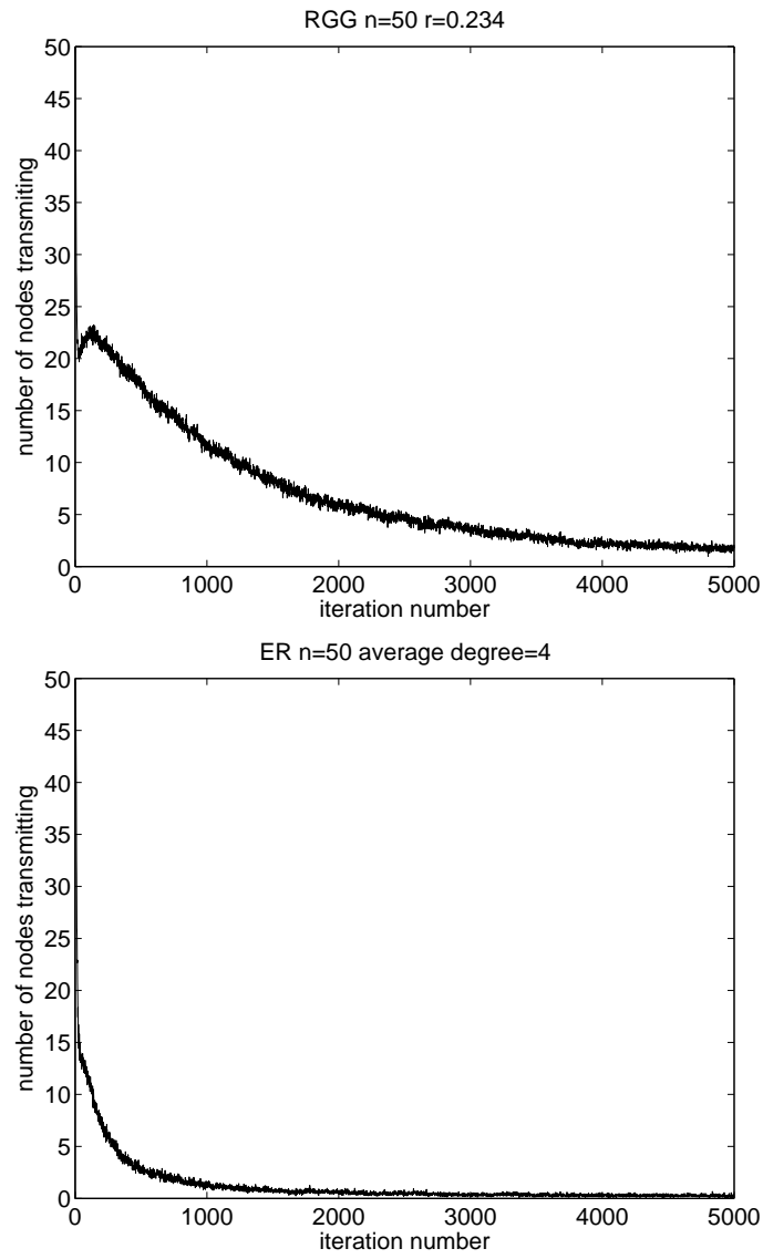
Figure 4: Messages sent with every iteration.
