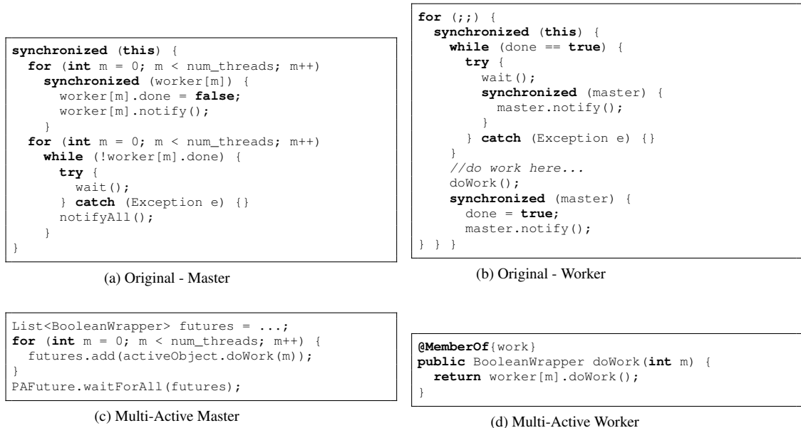
Figure 8: NPB master-worker paradigm original and multi-active version
