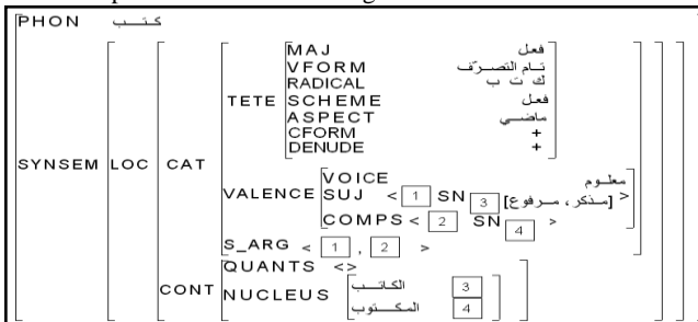
Figure 9: AVM of the verb kataba
