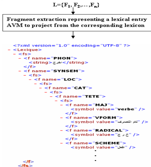
Figure 17: XML fragment extraction of a lexical entry in conformity with ISO 24610-1
