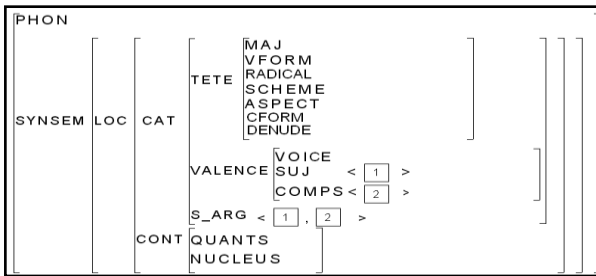
Figure 8: Model of an AVM of a verb
