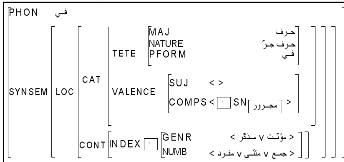
Figure 7: AVM of the particle fī
