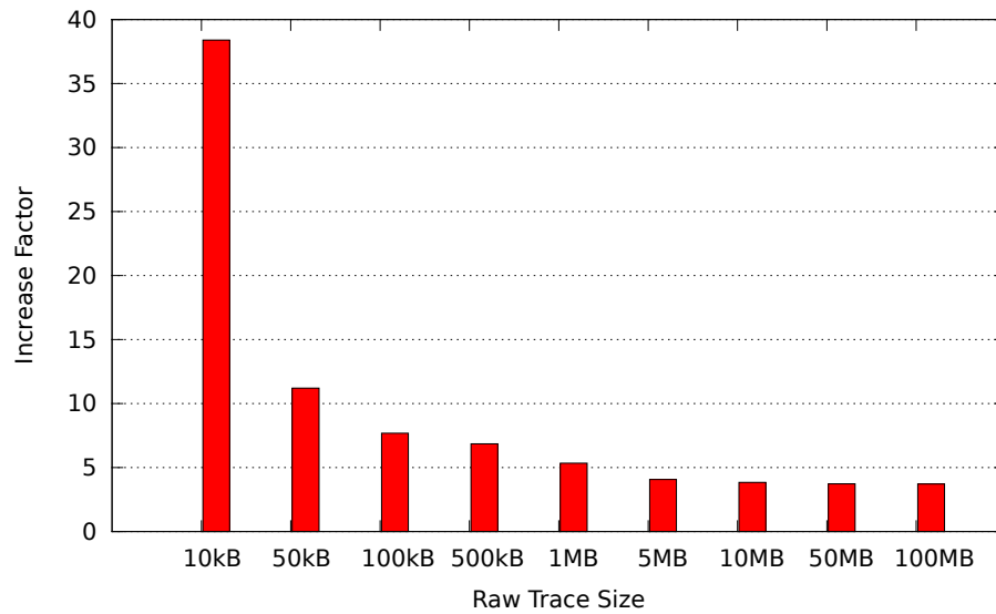
FIG. 19 – Database overhead
