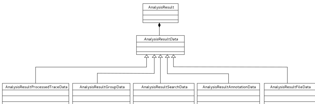
FIG. 13 – Analysis results class diagram
