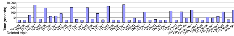
Figure 18: Schema triple deletion times.
