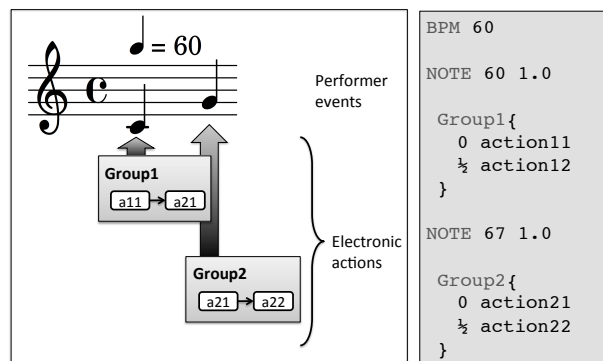
Figure 4. Sample score diagram and the corresponding simple Antescofo score
