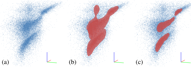
Fig. 10. CloudLasso being applied to a 3D scatter plot; data from a subset of the milliMillennium dataset [5] (showing the dimensions virial radius, R-I color, and low X-ray luminosity); (a) original 3D scatter plot, (b) initial CloudLasso selection, (c) after interactive threshold adjustment.
