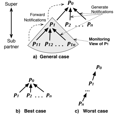
Figure 4. Super/Sub-Partner Tree
