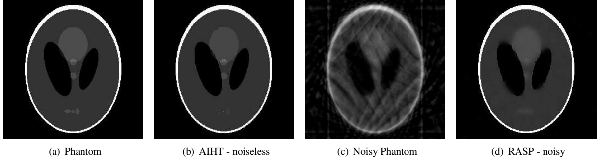
Figure 3: From left to right: Shepp Logan phantom image, AIHT reconstruction using 35 radial lines, noisy image with SNR of 20 and recovered image using RASP and only 22 radial lines. Note that for the noiseless case RASP and RACoSAMP get a perfect reconstruction using only 15 radial lines.
