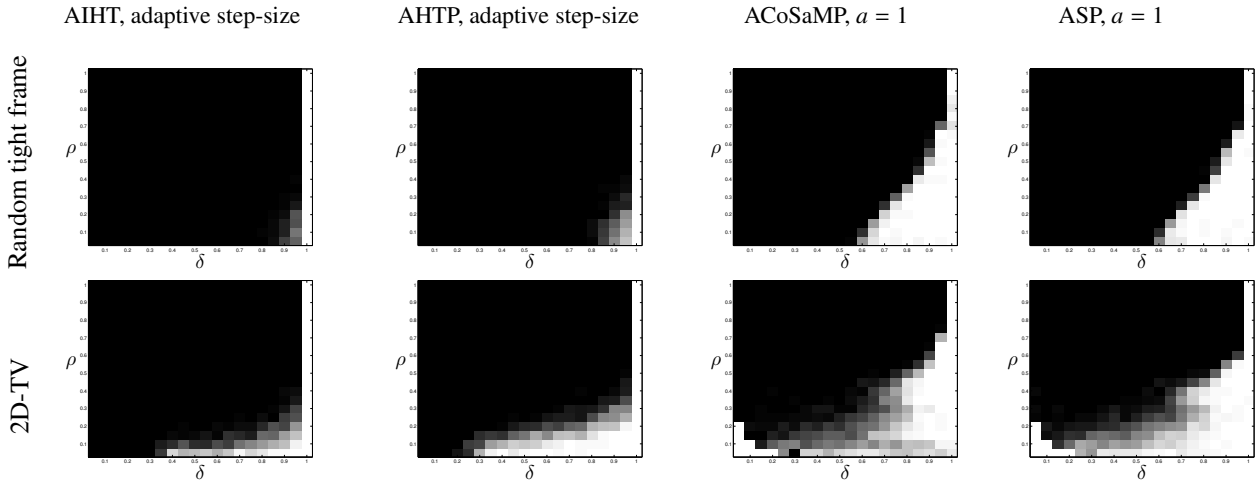
Figure 2: Recovery rate for a random tight frame with p = 240 and d = 120 (up) and a finite difference operator (bottom). From left to right: AIHT and AHTP with an adaptive changing step-size, and ACoSaMP and ASP with a = 1 .
