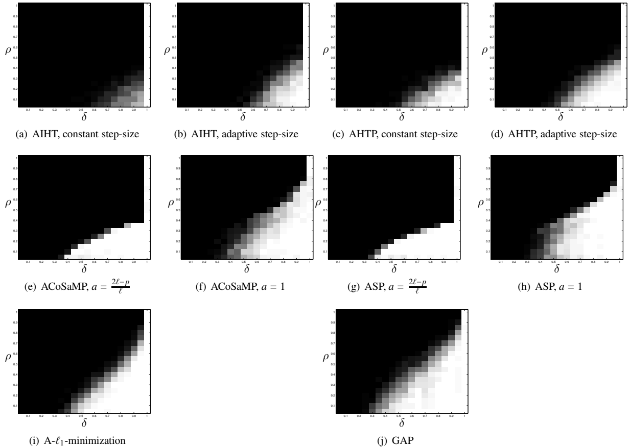
Figure 1: Recovery rate for a random tight frame with p = 144 and d = 120 . From left to right, up to bottom: AIHT with a constant step-size, AIHT with an adaptive changing step-size, AHTP with a constant step-size, AHTP with an adaptive changing step-size, ACoSaMP with a = \frac{2\ell-p}{\ell} , ACoSaMP with a = 1 , ASP with a = \frac{2\ell-p}{\ell} , ASP with a = 1 , A\text{-}\ell_1 -minimization and GAP.
