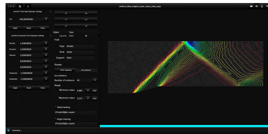
Figure 15: Pressure field: shock wave reflecting.
