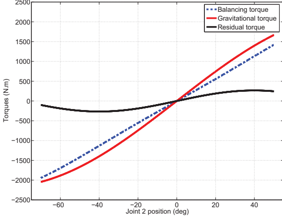
Fig. 5. Balancing system (upper) and Gravitational, Balancing and Residual torques (below)
