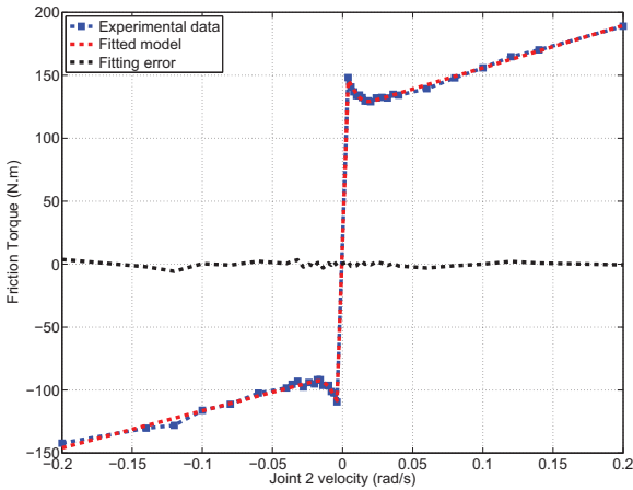
Fig. 6. Experimental friction torque and fitted Stribeck curve
