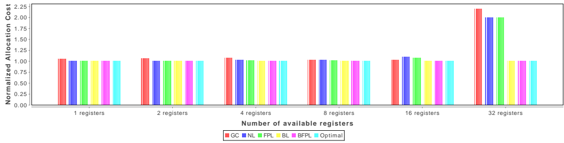
Figure 10: Allocation cost for the LAO-KERNELS benchmark suite on ARMv7.
