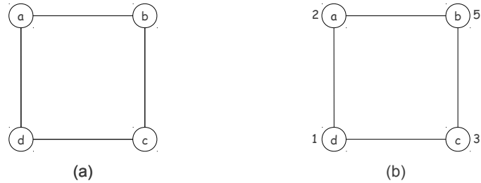
Figure 3: (a) An arbitrary graph. (b) A weighted graph.
